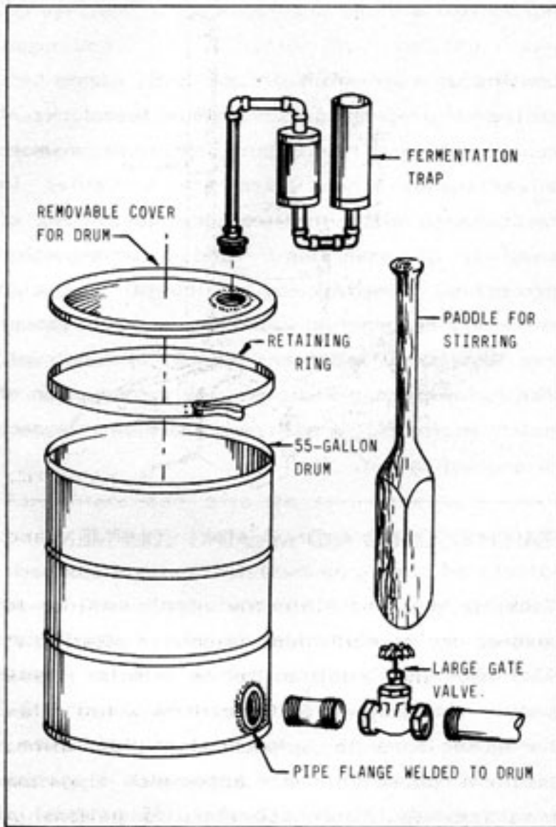
Figure 13-1: SMALL APPARATUS
