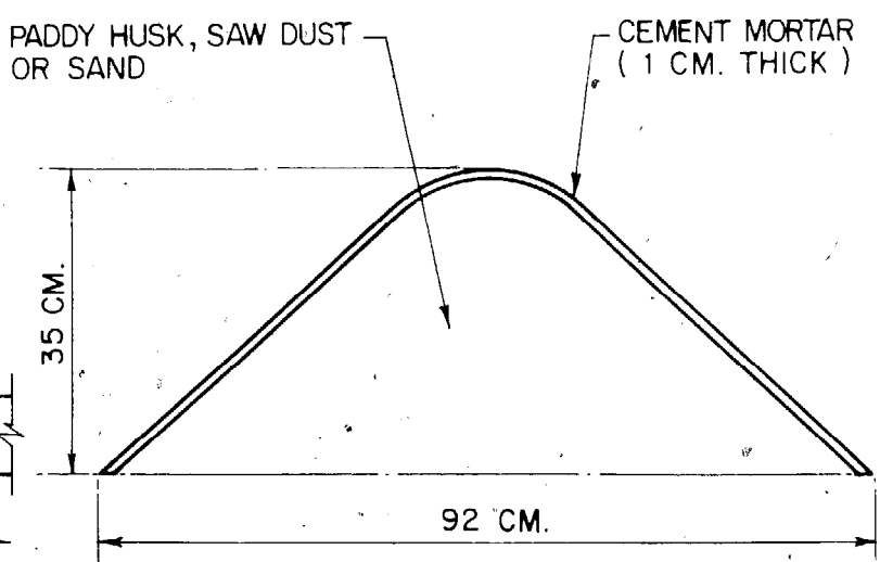
DETAIL OF CAP
