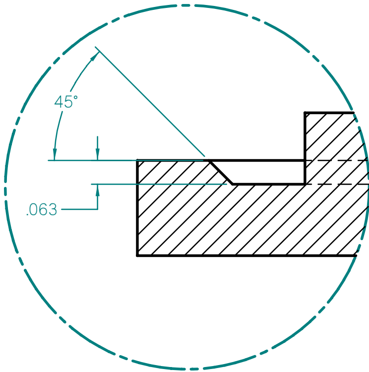
DETAIL B 4:1
