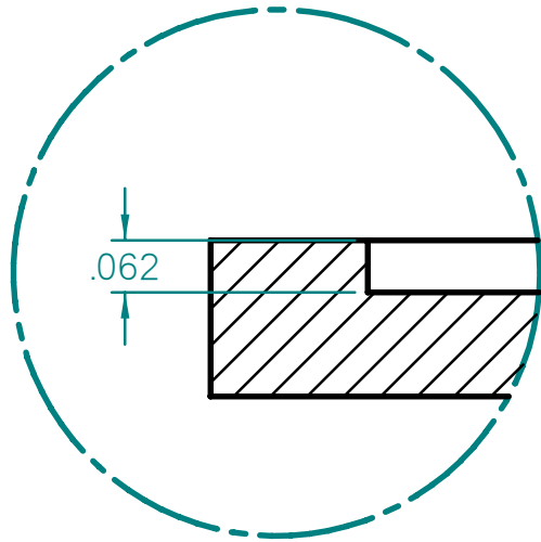
DETAIL B 4:1
